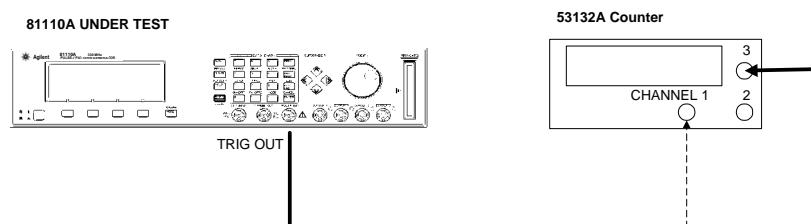
Connecting Agilent 81110A to the Counter
